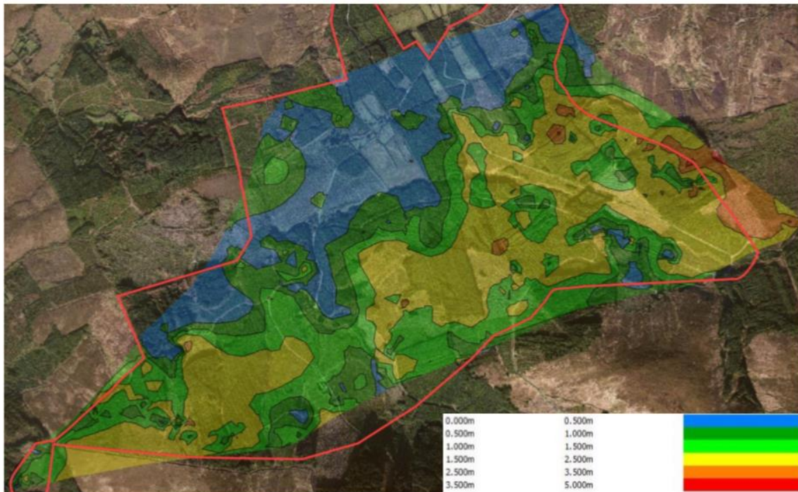
Figure 9.3: Peat Depth Map (Wind Farm)
