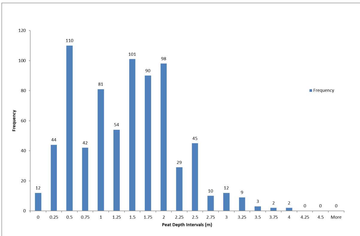
Figure 9.4: Peat depth frequency distribution plot
